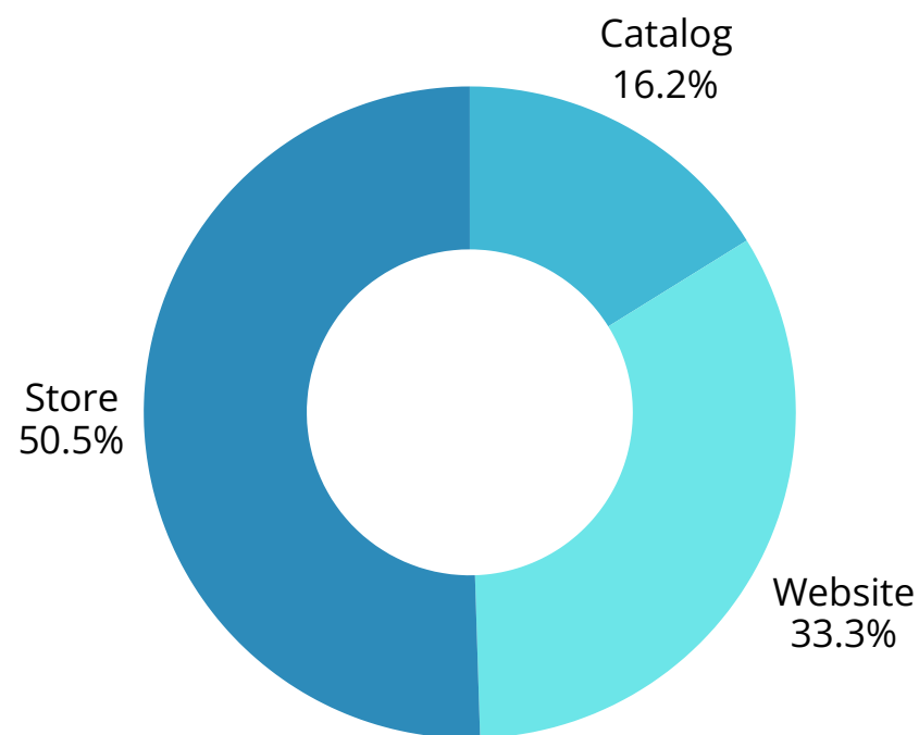
Channels Distribution
